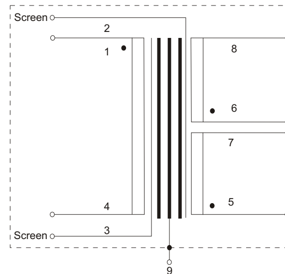
Electrical schematic
